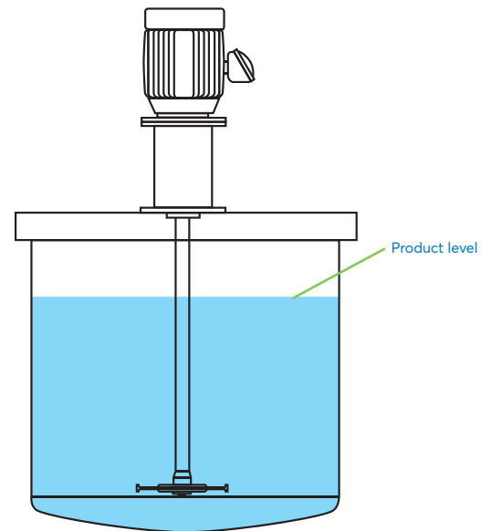
FIGURE 7: Tank Configuration Allow 10 hp per 100 gallons of product. Single shaft dispersers are not recommended for products over 50,000 cps.
