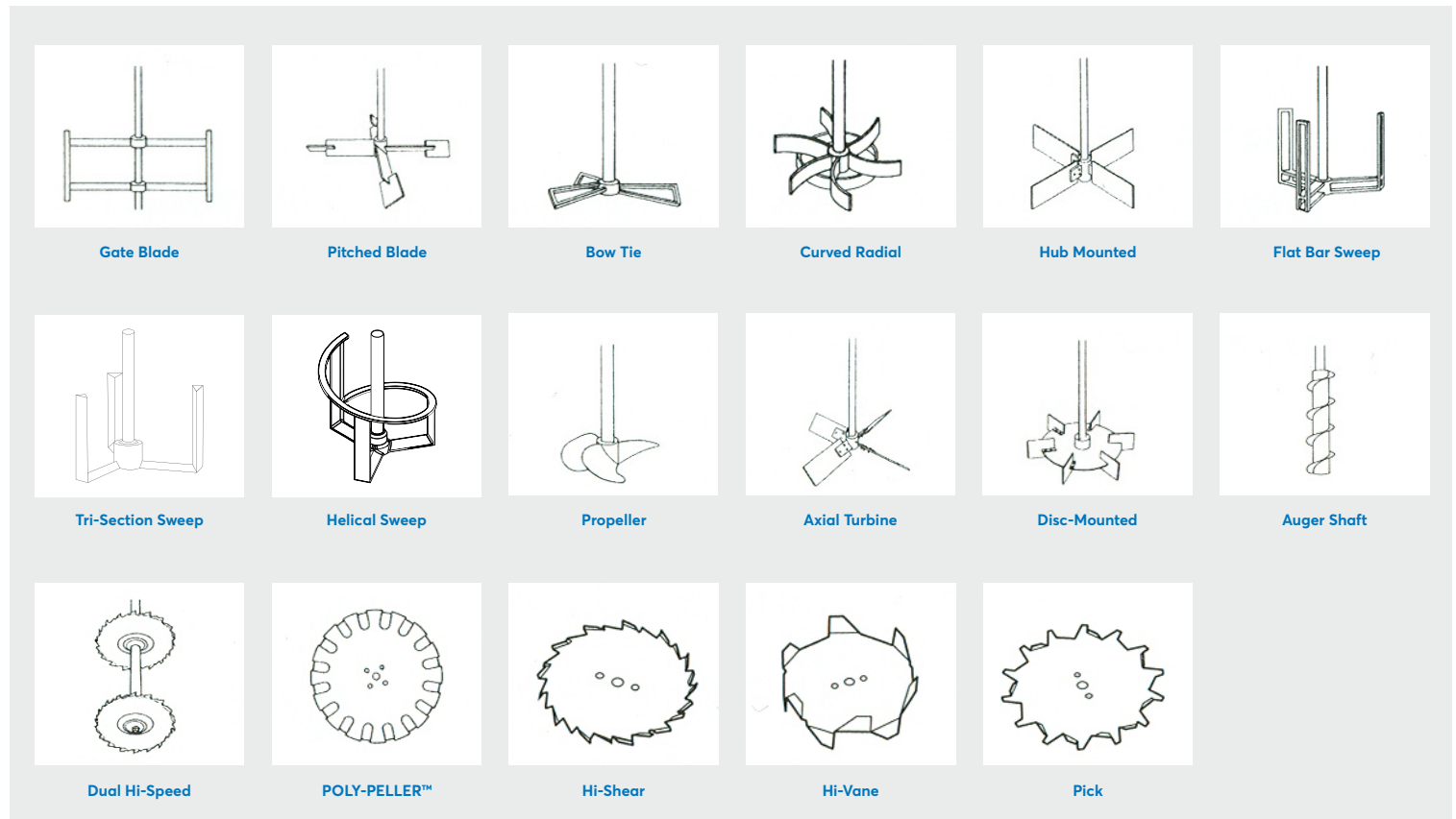
FIGURE 5: Impeller Designs
